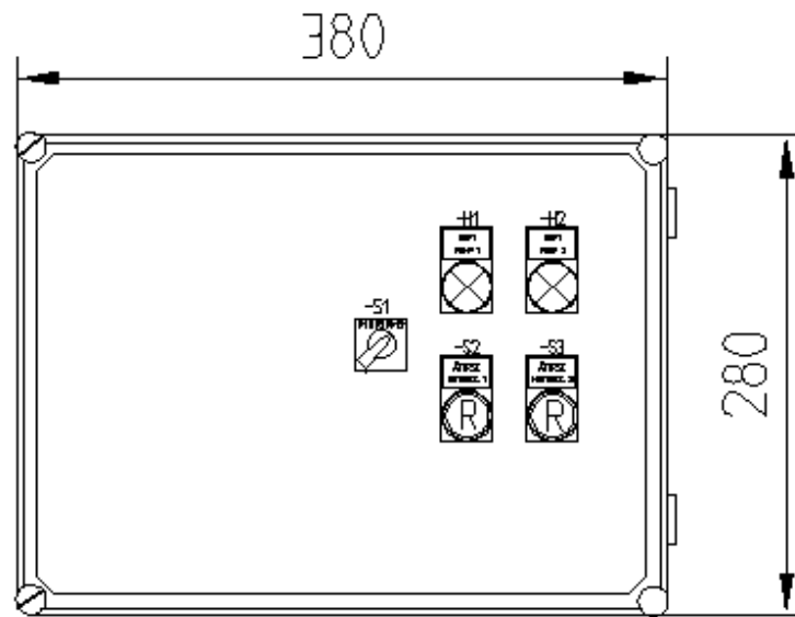
FIBOX PG382818
